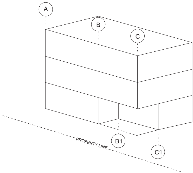
FIGURE I704.8b ISOMETRIC VIEW
