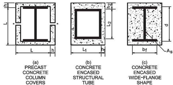
FIGURE 721.5.1(6) CONCRETE PROTECTED STRUCTURAL STEEL COLUMNS a,b
